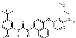
1-(5-tert-Butyl-2-methoxy-phenyl)-3-{4-[2-(2-methoxy-ethyl-amino)-pyrimidin-4-yloxy]-naphthalen-1-yl}-urea;
